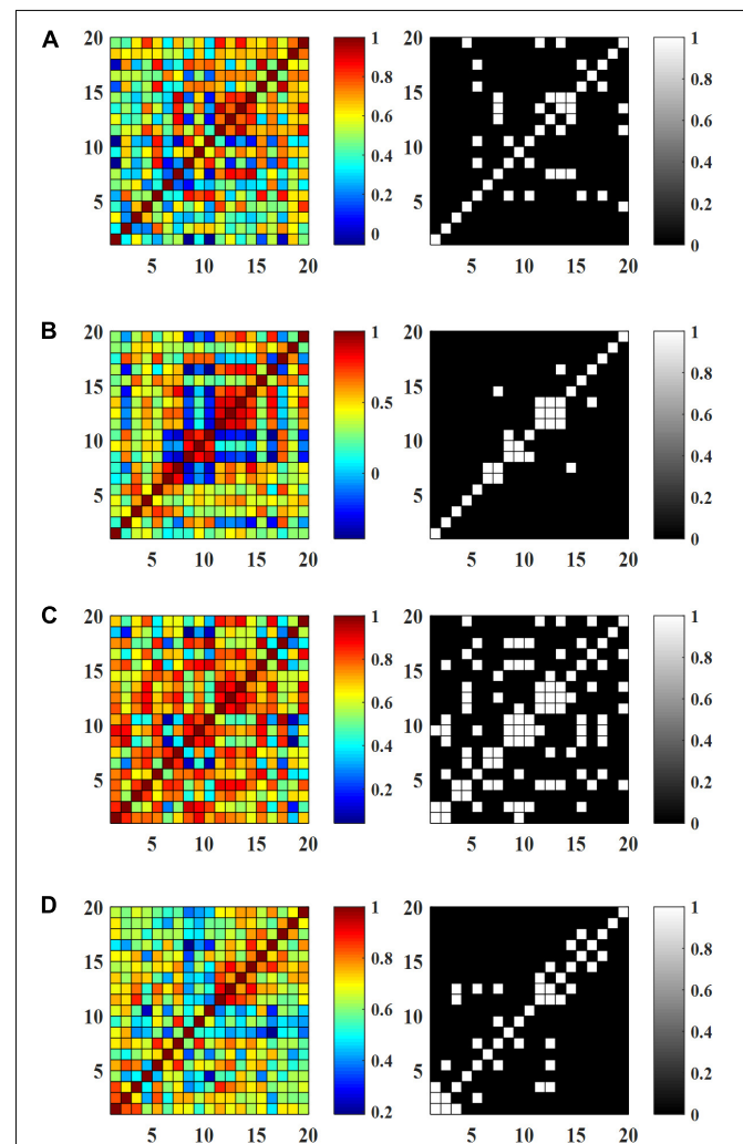
FIGURE 6 | Resting state functional connectivity and the corresponding binary matrices (threshold value 0.8): (A) HC, (B) MCI-0, (C) MCI-1, and (D) MCI-2.
