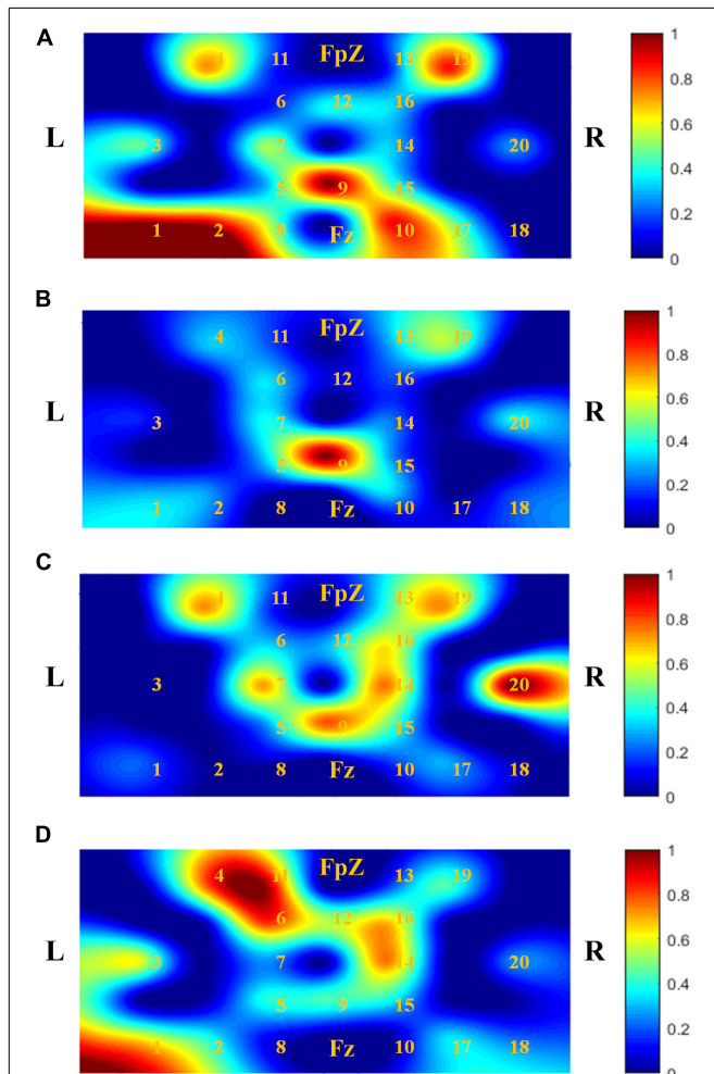
FIGURE 5 | Comparison of activation patterns ( t -maps) of \Delta\text{HbO} s averaged over all subjects and trials: (A) t -map of HC, (B) MCI-0 [baseline, before acupuncture therapy (AT)], (C) MCI-1 (after 12 sessions of AT for 6 weeks), and (D) MCI-2 (after another 12 sessions of AT for 6 weeks). It is seen that AT makes the activated brain region wider.
