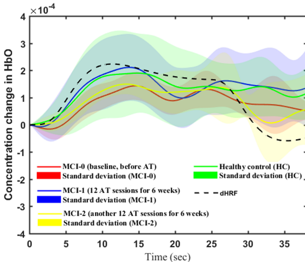
FIGURE 4 | Averaged \Delta\text{HbO} s (solid lines) and their standard deviations (shaded region) of HC, MCI-0, MCI-1, and MCI-2 (the dashed curve denotes the dHRF).
