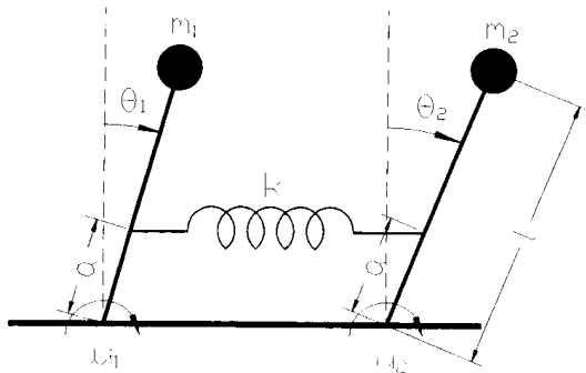
Fig. 1 Inverted double pendulums
