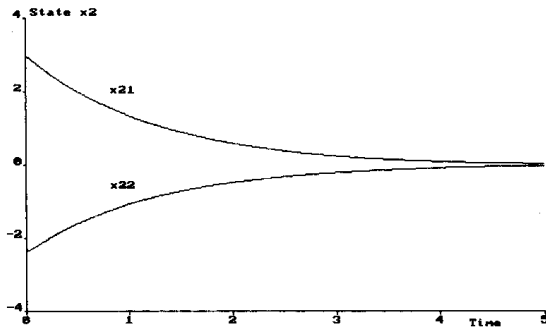
Fig. 3 State history of subsystem 2
